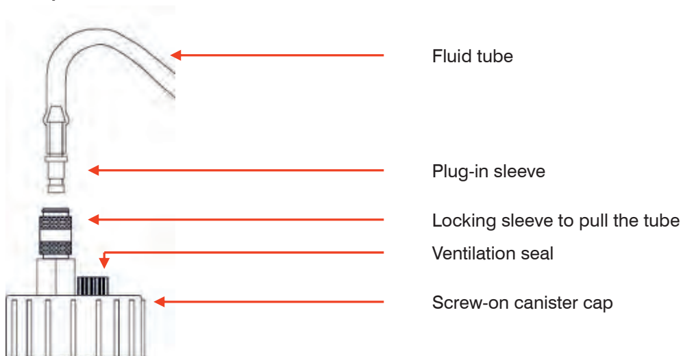
Canister cap of the fluid
